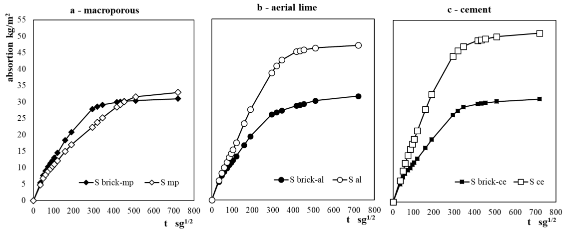
Fig. 2. Graphs of the absorption test results.
