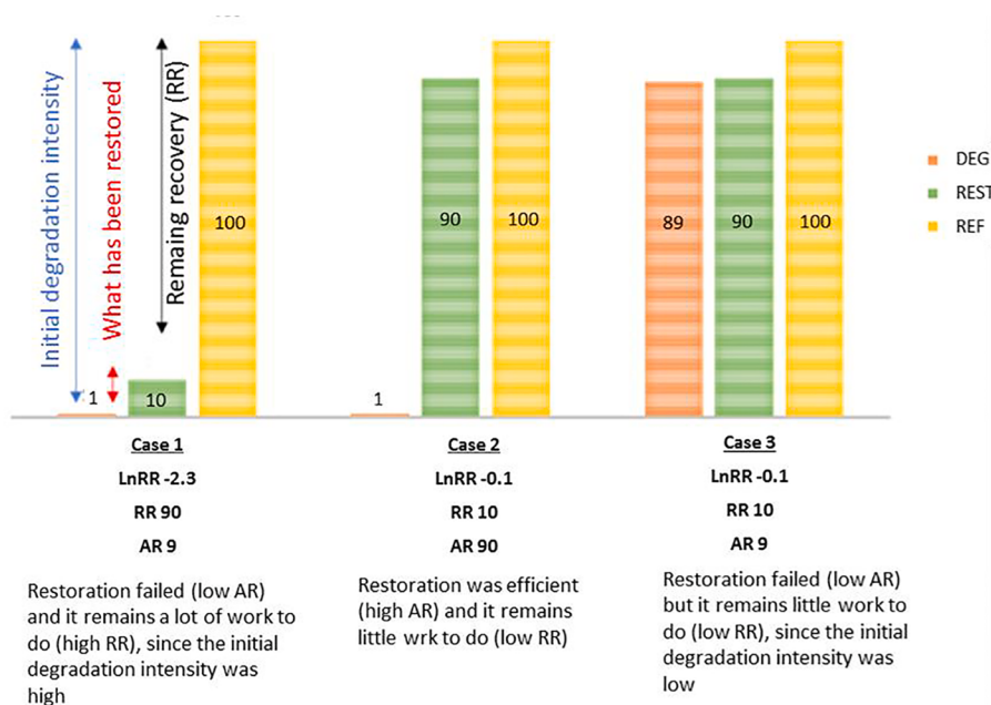
Fig. 2. Graphical illustration of how the AR index (Achieved Restoration, %) complements the LnRR index (Remaining Recovery). Case studies correspond to theoretical situations. Red, green and yellow bars, respectively, represent the degraded (Deg), Restored (Rest) and Reference (Ref) states. LnRR corresponds to \ln(\text{Rest}/\text{Ref}) , RR (%) is calculated as 100 \times (1 - e^{\ln \text{LnRR}}) , and AR as 100 \times [(\text{Rest}-\text{Deg})/(\text{Ref}-\text{Deg})] . The three case studies correspond to situations where the restoration operation (here ER + ) correctly worked (see Table 1). (For interpretation of the references to colour in this figure legend, the reader is referred to the web version of this article.)
