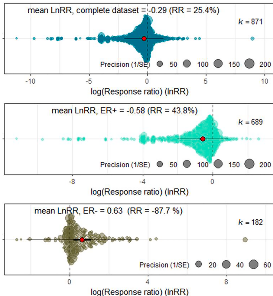
Fig. 1. Distribution of effect sizes estimating the success of ecological restoration actions as the log-response ratio between ecosystem attributes in restored vs. reference states. From top to bottom: Whole dataset ( n = 871 ), ecological restoration actions aiming at increasing ( ER^+ , n = 689 ) or decreasing ( ER^- , n = 182 ) the levels of ecosystem attributes. The x-scale is not always centered in the same way between the three panels.
