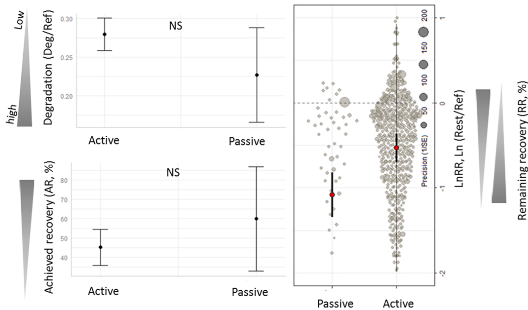
Fig. 3. Coefficient parameter estimates ( \pm 95\% CI represented by bars) of models decoupling active and passive restorations. Top left: initial degradation level (glm model), bottom left: Achieved recovery, AR (glm model), right: Log ratio of Remaining recovery, LnRR (rma.mv model). Grey arrows indicate the level of the three indices. For LnRR, a fourth arrow informs on the resulting remaining recovery (RR). NS: non-significant.
