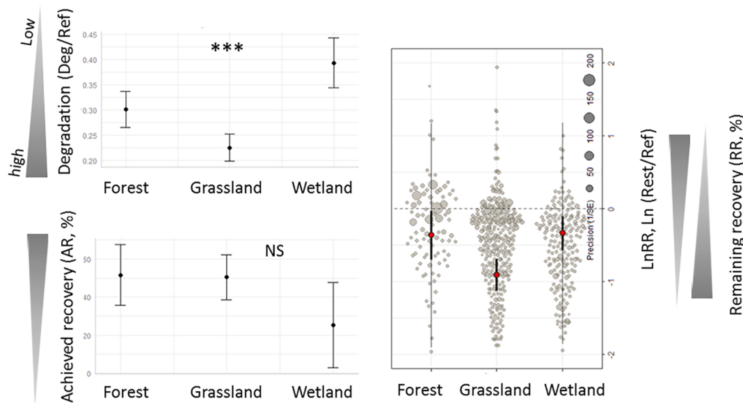
Fig. 5. Coefficient parameter estimates ( \pm 95\% CI represented by bars) of models decoupling the habitat types where restoration was implemented. Top left: initial degradation level (glm model), bottom left: Achieved recovery, AR (glm model), right: Log ratio of remaining recovery, LnRR (rma.mv model). Grey arrows indicate the level of the three indices. For LnRR, a fourth arrow informs on the resulting remaining recovery (RR). NS: non-significant, ***: p < 0.001 .
