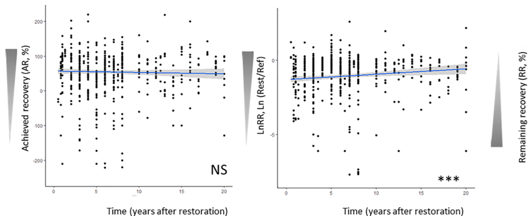
Fig. 4. Relationship (linear regression, \pm 95\% CI) between the achieved recovery, AR (left), or the Log ratio of Remaining recovery, LnRR (right), and the time elapsed since the restoration operation started (x-axis). Grey arrows indicate the level of both indices. For LnRR, a fourth arrow informs on the resulting remaining recovery (RR). NS: non-significant, ***: p < 0.001 .
