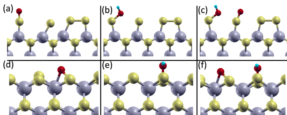
Fig. 6. Adsorption geometries on the edges of the \text{MoS}_2 layer. (a)–(c) Mo-edge (d)–(f) S-edge.
