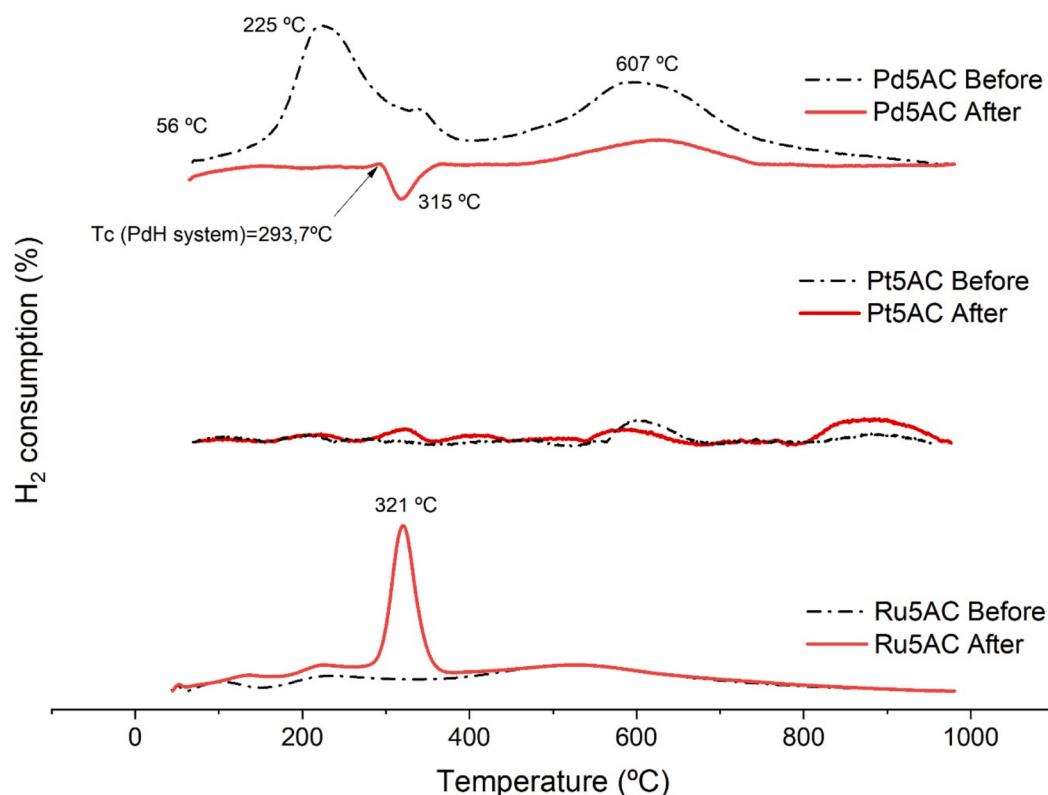
Fig. 6. H 2 -TPR curves of catalysts Pd5AC, Pt5AC and Ru5AC before and after reduction of carbamate with pure-hydrogen. Reaction conditions: 2 h, 2.5 MPa of 99.99 % pure-hydrogen, catalyst metal:carbamate molar ratio of 3.8 mmol, 70 % of filling and 0.5 M of initial concentration.
