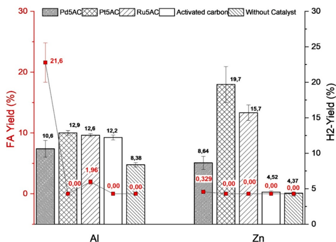
Fig. 3. FA and H 2 yield for the different metal/catalyst systems. Reaction conditions: 2 h, metal:carbamate molar ratio of 6, catalyst metal:carbamate molar ratio of 3.8 mmol, 70 % of filling and 0.5 M of initial concentration.
