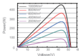
Power-Voltage Curve JAM78S10-435/MR
