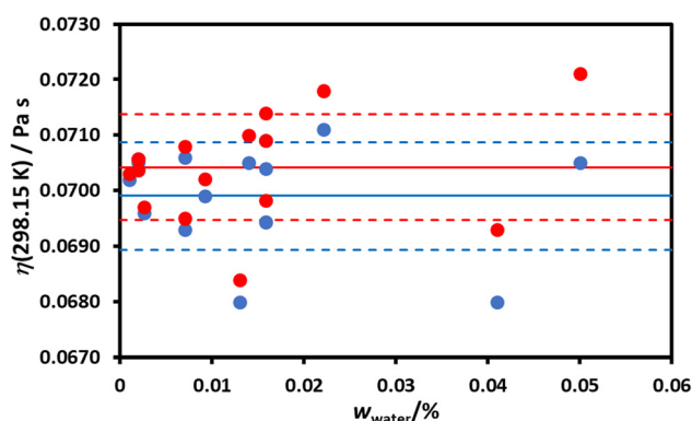
FIG. 17. The viscosity of [\text{C}_6\text{mim}][(\text{CF}_3\text{SO}_2)_2\text{N}] at 298.15 K obtained from different sets of water-free primary data as a function of the water content of the measured samples (in red). Also shown, for comparison, is the result that we would have obtained if the raw data were used (in blue).
