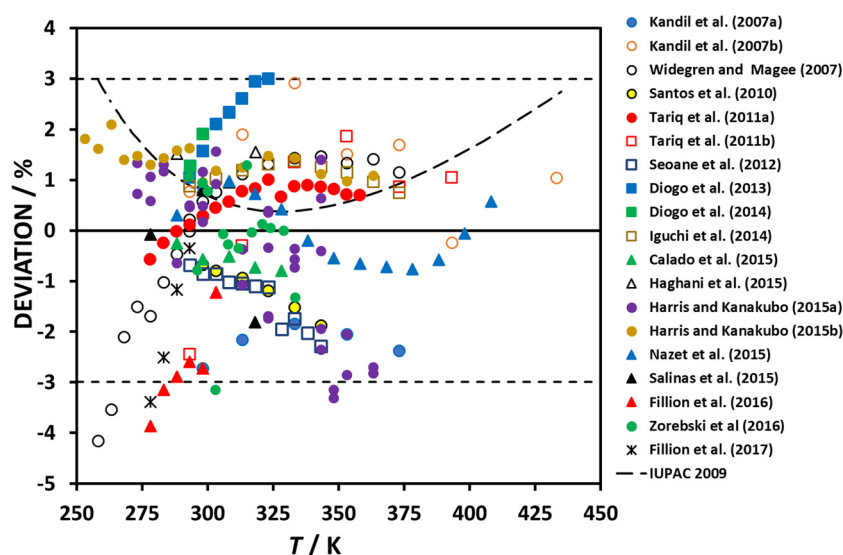
FIG. 18. Deviations between the primary data for the viscosity of [\text{C}_6\text{mim}][(\text{CF}_3\text{SO}_2)_2\text{N}] as a function of temperature. The dashed line represents the uncertainty of the correlation of \pm 3.0\% .
