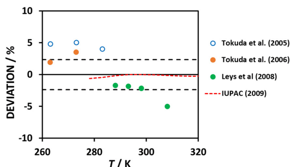
FIG. 23. Deviations of the secondary data for the electrical conductivity of [\text{C}_6\text{mim}][(\text{CF}_3\text{SO}_2)_2\text{N}] from the proposed reference correlation as a function of temperature. The dashed line represents the uncertainty of the correlation at a 95% confidence level (2.4%). Also shown is the IUPAC (2009) correlation. 4
