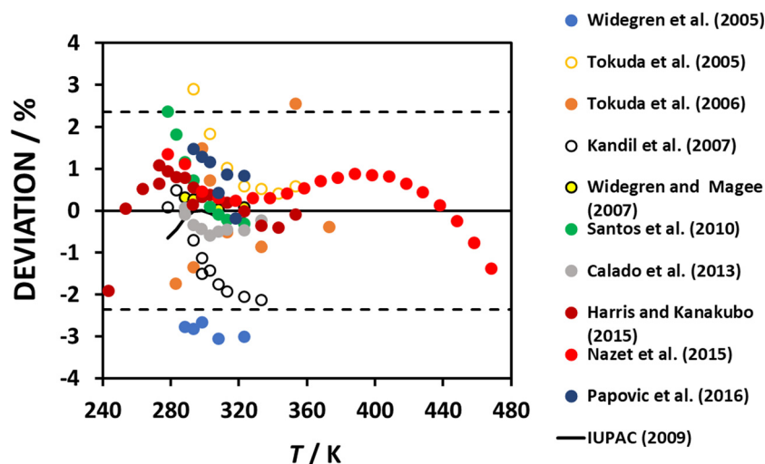
FIG. 22. Deviations of the primary data for the electrical conductivity of [\text{C}_6\text{mim}][(\text{CF}_3\text{SO}_2)_2\text{N}] from the proposed reference correlation as a function of temperature. The dashed line represents the uncertainty of the correlation at a 95% confidence level (2.4%). Also shown is the IUPAC (2009) correlation. 4
