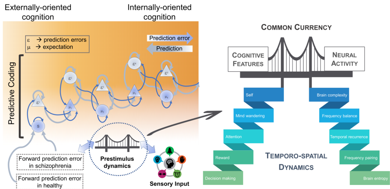
Figure 4. Relevance of temporospatial dynamics in cognition. Temporospatial dynamics during the prestimulus provide a bridge of neuronal and mental activity serving as “common currency”. The altered neural dynamics in schizophrenia is received by predictive coding modeling as the forward prediction error input, ultimately affecting the internally-oriented cognition.
