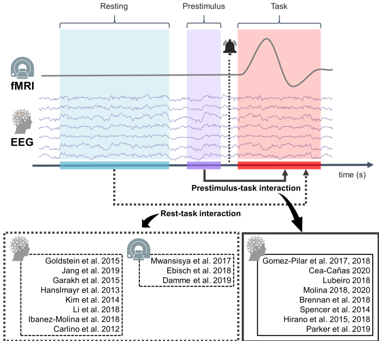
Figure 1. Overview of the study. We reviewed studies that directly analyzed rest-task interaction or prestimulus-task interaction, both in EEG and fMRI modalities.
