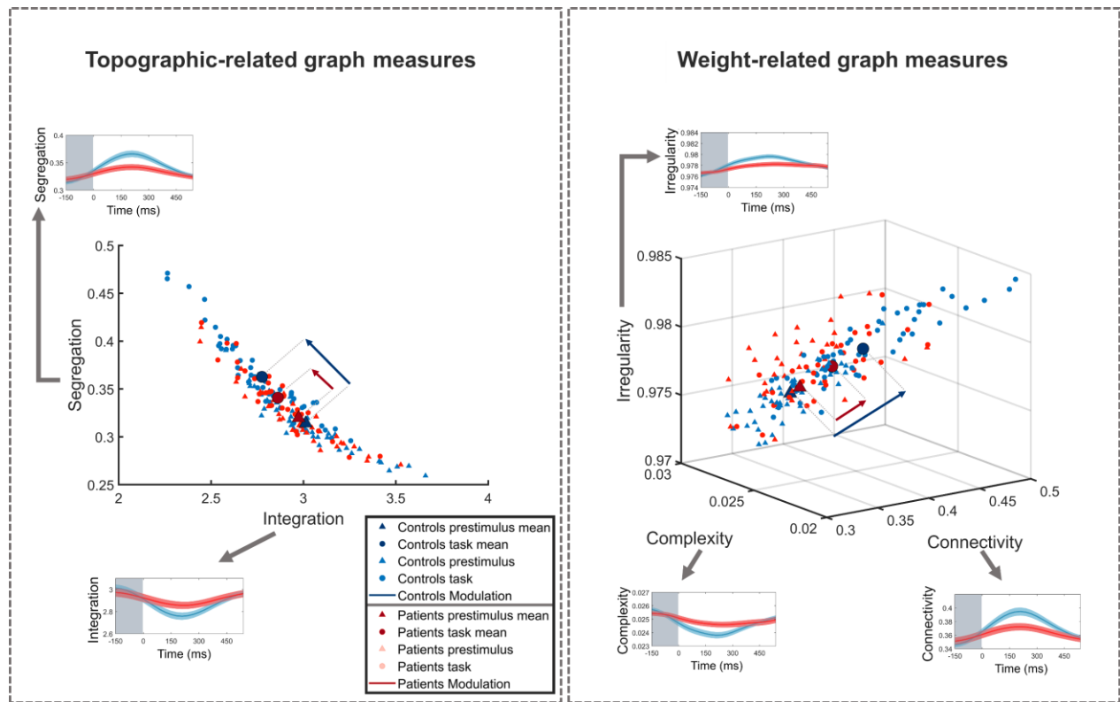
Figure 2. Temporospatial dynamics of chronnectomic measures during prestimulus-task modulation in healthy and schizophrenia subjects. Schizophrenia subjects show reduced temporospatial dynamics both for the topographic-related graph measures (A) and for the weight-related graph measures (B). In the bottom row (C and D), the modulation from prestimulus to task-related activity is depicted with a blue line for controls and red line for patients, showing reduced
