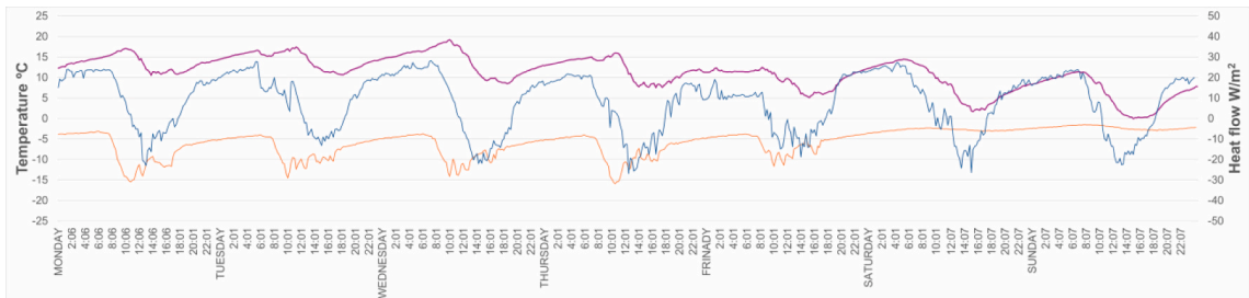
Fig. 8. Representation of the heat flows measured by the plates and according to Fourier's Law during a winter week (11–17/03/24) Theoretical heat flow according to Fourier's Law (W/m²) FiP= Heat flux measured by the plate placed on the interior face of the wall (W/m²) FeP= Heat flux measured by the plate placed on the exterior face of the wall (W/m²).
