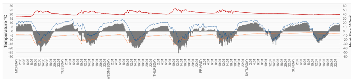
Fig. 10. Inside ambient temperature and heat flux during a winter week (11–17/03/24) Ta = Indoor ambient temperature measured by the probe ( ^{\circ}C ) FiP = Heat flux measured by the plate placed on the interior face of the wall ( W/m^2 ) FeP = Heat flux measured by the plate placed on the exterior face of the wall ( W/m^2 ) FiP + FeP = Sum of the heat flows measured by both plates ( W/m^2 ).
