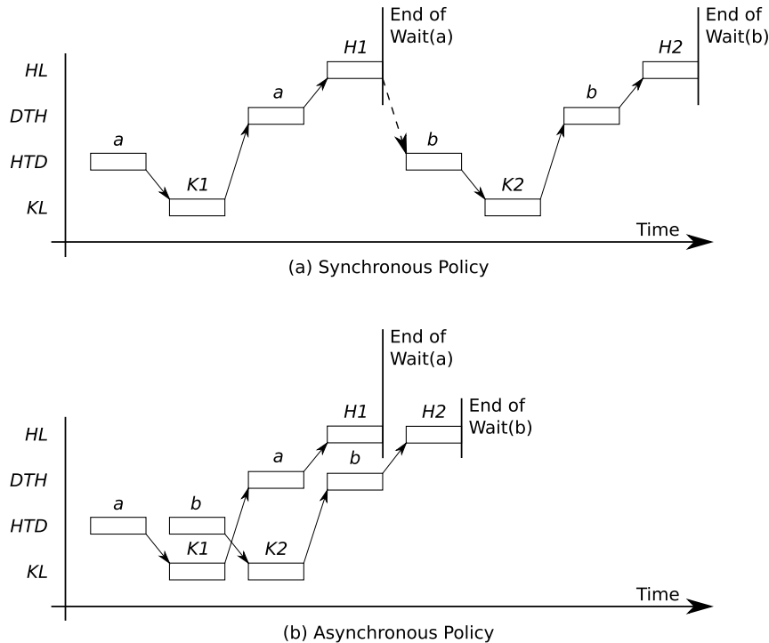
Fig. 5. Execution of a set of operations in synchronous (top) and asynchronous (bottom) execution models.
