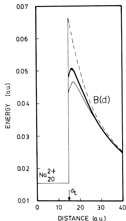
FIG. 3. Calculated capture barrier B(d) for the reaction \text{Na}_{19}^+ + \text{Na}^+ \rightarrow \text{Na}_{20}^{2+} . Dashed line, pure Coulomb approximation; thick solid line, extended Thomas-Fermi barrier; thin solid line, classical conducting-sphere model. Notice that the fission barrier F(d) is obtained by measuring B(d) from the ground-state energy of \text{Na}_{20}^{2+} [see Eq. (5)] which is indicated by a horizontal line on the left.
