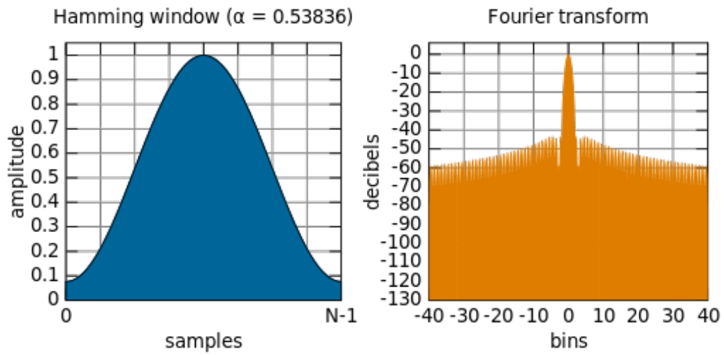
Figura 2.7: Ventana de Hamming.
