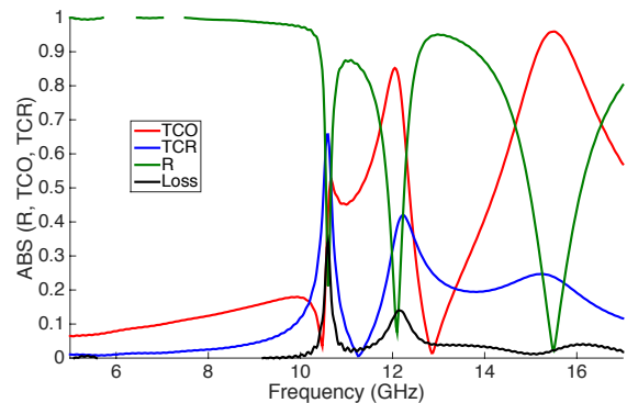
Figure 4: Reflection ( R ), Copolarization ( T_{CO} ), and Crosspolarization ( T_{CR} ) transmission coefficients, as well as relative losses for a plane wave normally incident over a periodic structure composed by cells as shown in Fig. 2. The dielectric slab is 0.03 inches width and it is made of Taconic TLC 30.
