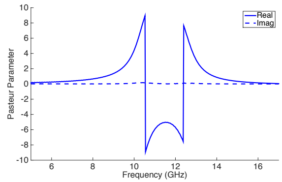
Figure 7: Effective Pasteur parameter ( \kappa ) of a periodic structure composed by cells like shown in Fig. 1. The dielectric slab is 0.03 inches width and it is made of Taonic TLC 30.
