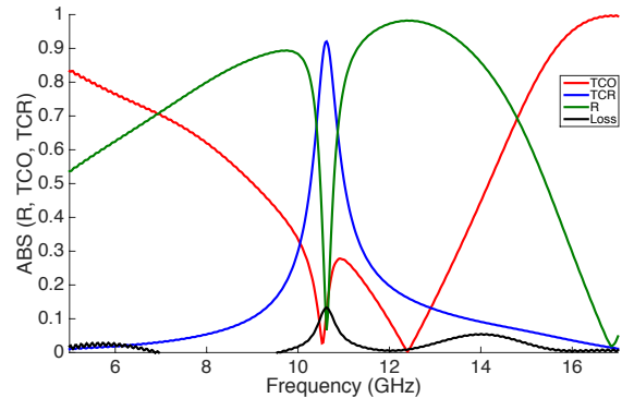
Figure 3: Reflection ( R ), Copolarization ( T_{CO} ), and Crosspolarization ( T_{CR} ) transmission coefficients, as well as relative losses for a plane wave normally incident over a periodic structure composed by cells as shown in Fig. 1. The dielectric slab is 0.03 inches width and it is made of Taconic TLC 30.
