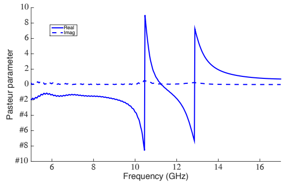
Figure 8: Effective Pasteur parameter ( \kappa ) of a periodic structure composed by cells like shown in Fig. 2. The dielectric slab is 0.03 inches width and it is made of Taonic TLC 30.
