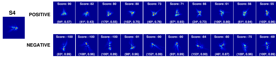
Figure 9.5: Example of the 10 top positively and negatively ranked PSFs for subject S4. The labels show the score and the parameters of the fitted ellipse (axis, eccentricity).
