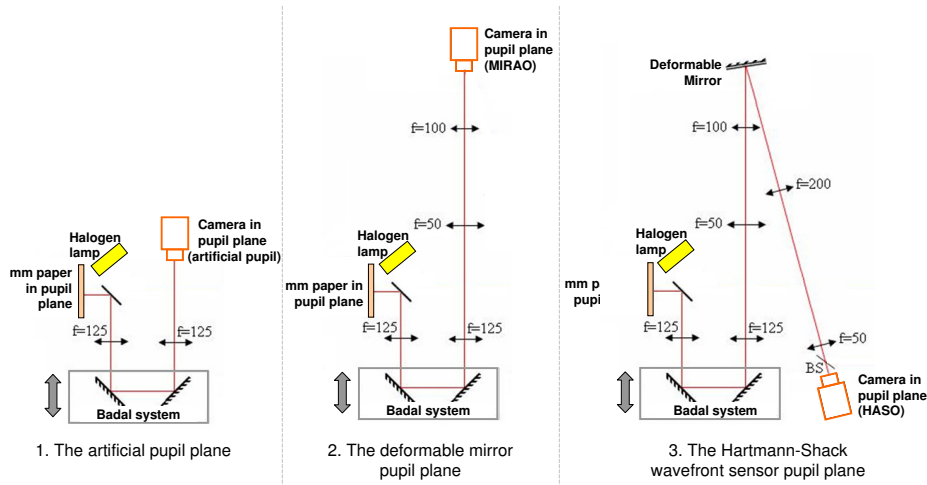
Figure 2.9: Illustration of the schematic configuration of the camera in each pupil plane used to check the constant magnification (artificial pupil (x1); MIRAIO deformable mirror (x2) and HASO HS sensor (x0.5)) regardless the Badal system position.
