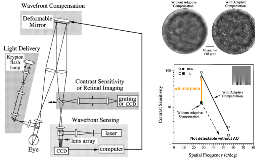
Figure 1.21: Wavefront sensing and adaptive compensation system developed in 1997, with an improvement in contrast sensitivity (for two eyes for horizontal grating of 27.5 and 55 c/deg) and higher contrast images of the cones mosaic (image of the retina at 4-deg eccentricity for one subject) with adaptive compensation, adapted from Liang et al. [1997].
