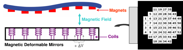
Figure 2.4: Magnetic deformable mirror (Adapted from Hampson [2008]) and the schematic representation of the MIRA052 (Imagine Eyes, France)
