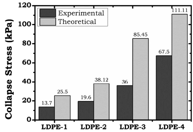
Fig. 8. Experimental and theoretical values of collapse stress.
