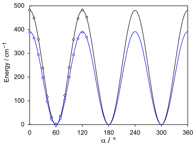
Figure 2: The potential energy curves of 2-chloro-4-fluorotoluene obtained by rotating the methyl group around the C3–C7 bond in 10° steps calculated at the MP2/6-311++G(2d,2p) (black curve) and B3LYP/6-311++G(2d,2p) levels of theory (blue curve) levels of theory. Only the V_3 term was adjusted to fit the calculated energies. The predicted potential barriers are 481.1 cm -1 and 391.5 cm -1 , respectively
