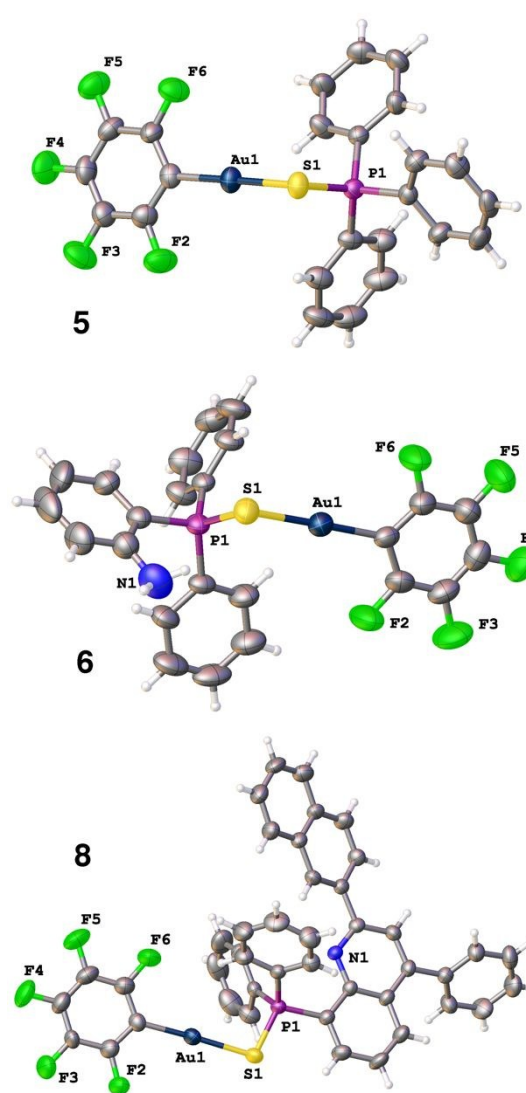
Figure 3. ORTEP view of molecular structure of complexes 5 , 6 and 8 with thermal ellipsoids at 50% probability.
