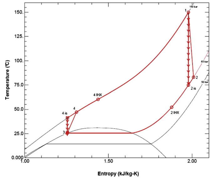
Fig. 3. T–s Diagram for different CO 2 transcritical power cycles.
