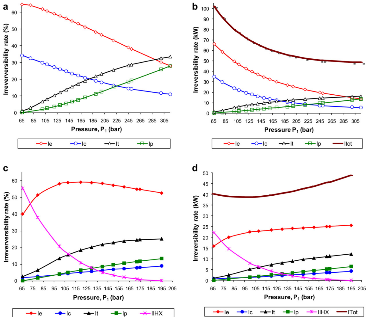
Fig. 8. Effect of the input pressure in the turbine over the irreversibilities of the process in an input temperature to the turbine at 150 °C for the cycle without IHX (a), (b) and for the cycle with IHX (c), (d).
