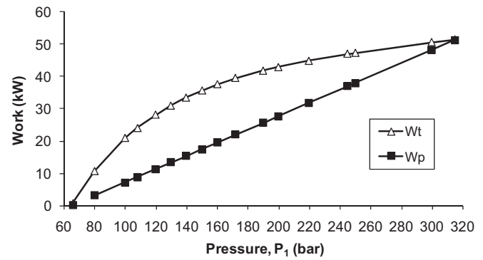
Fig. 6. Work produced and consumed by the turbine and the pump, respectively vs Pressure P_1 at T_1 = 150 °C, without IHX.
