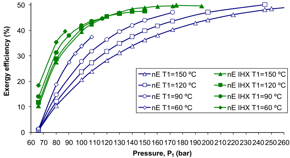
Fig. 9. Exergy efficiency vs Pressure P 1 with and without IHX and for the studied temperatures.
