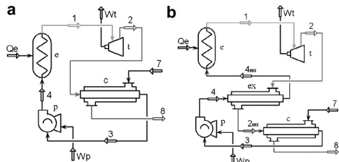
Fig. 2. Schematics diagram of the process simple (a) and with IHx (b). (t) Turbine, (c) Condenser, (p) Pump, (e) Evaporator, (ex) Internal Heat Exchanger.
