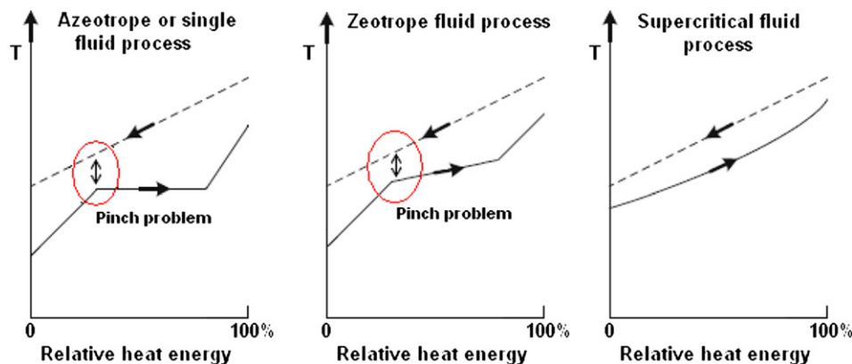
Fig. 1. Schematic diagram of the temperature variation between heat source (---) and working fluid (—) in the counter current evaporator for azeotrope or single fluid, zeotropic and supercritical process, respectively.
