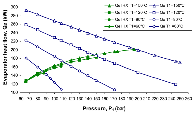
Fig. 7. Heat required in the evaporator vs. input pressure to the turbine P 1 for each one of the temperatures studied in the cycle with and without IHX.
