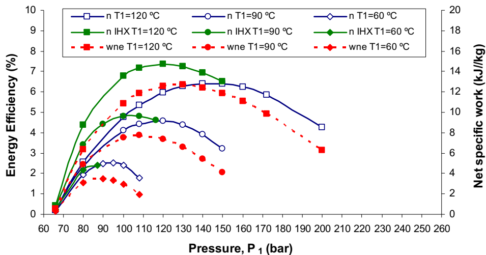
Fig. 5. Energy efficiency ( \eta ) with IHX (bold symbols) and without IHX (open symbols), and net specific work (wne) produced (discontinuous lines) vs. Pressure P_1 for T_1 = 120 °C (square), 90 °C (circle), and 60 °C (rhombus).
