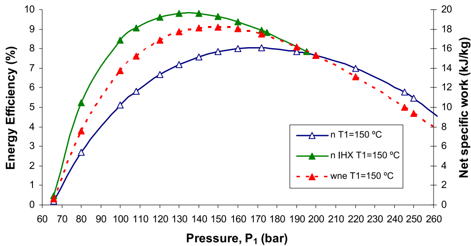
Fig. 4. Energy efficiency ( \eta ) with IHX ( \blacktriangle ) and without IHX ( \triangle ), and net specific work (wne) produced vs. Pressure P_1 for T_1 = 150 °C.
