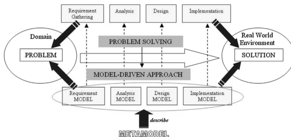
Figure 3. Problem-solving through the model-driven approach.
